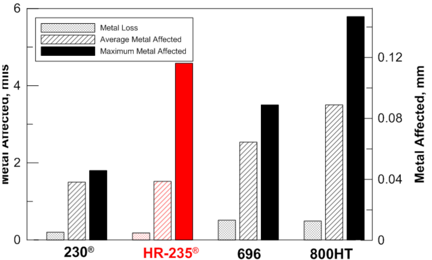
Oxidation Resistance at 1800°F (982°C)
