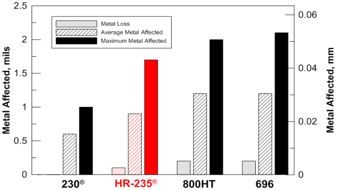
Oxidation Resistance at 1600°F (871°C)
